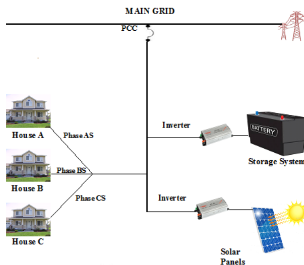
Fig. 1. The experimental microgrid setup
