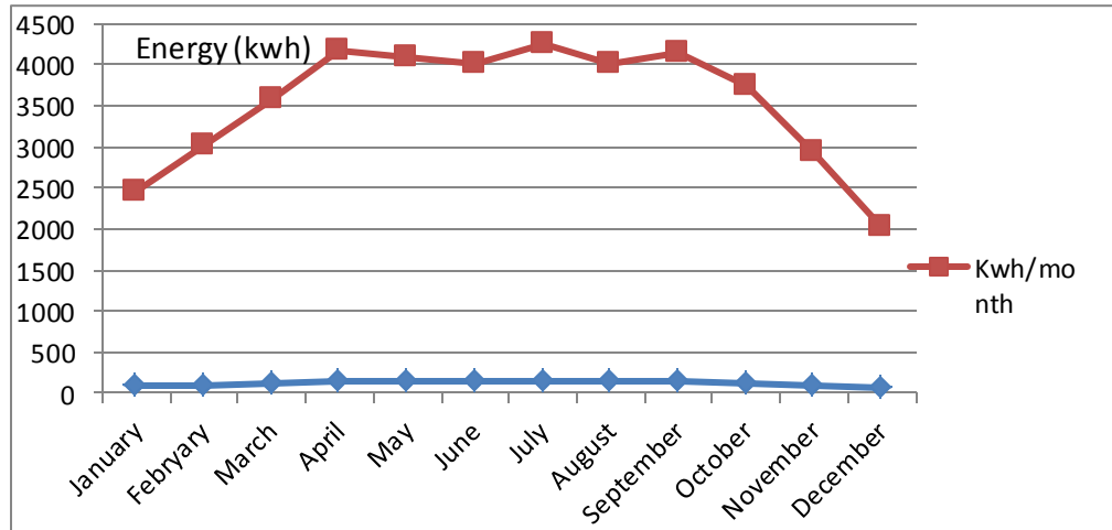
Figure 3 The amount of energy produced by solar panels
