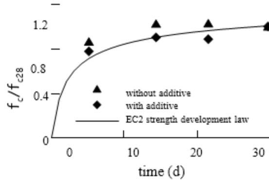
Figure 8. Strength development of concrete with and without crystalline additives vs. EC2 provisions
